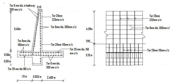
figure.3 details of cantilever retaining wall.
