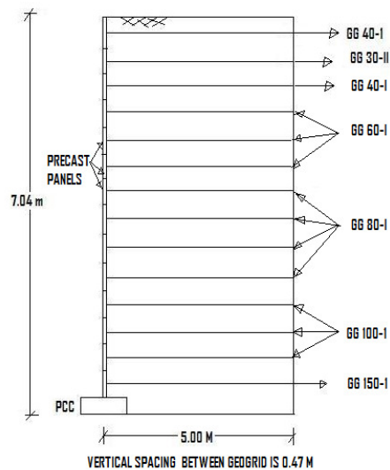
figure.2 details of reinforced earth wall.
