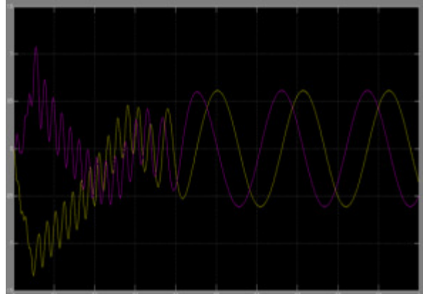
Fig.9 Rotor Flux \Phi_{ir-q,d}
