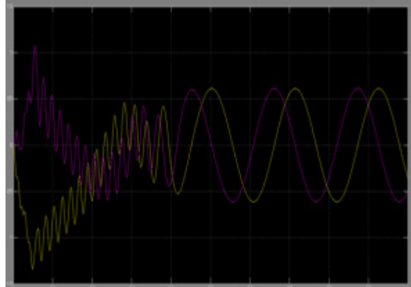
Fig.9 Rotor Flux Phir-q,d
