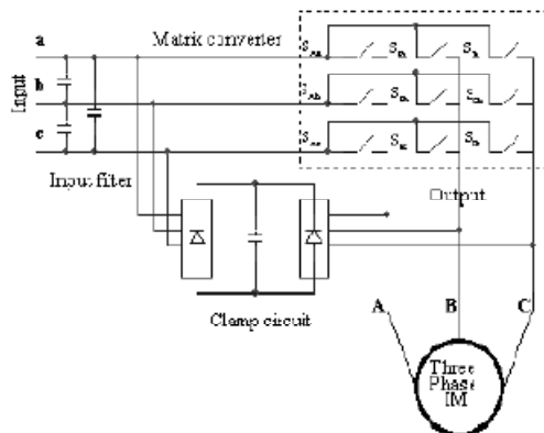
Fig.2 The practical scheme of matrix converter drive
