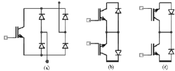
Fig.3 Bi-directional switch topologies using unidirectional switches: a) diode embedded; b) common emitter(CE); c) common collector(CC).
