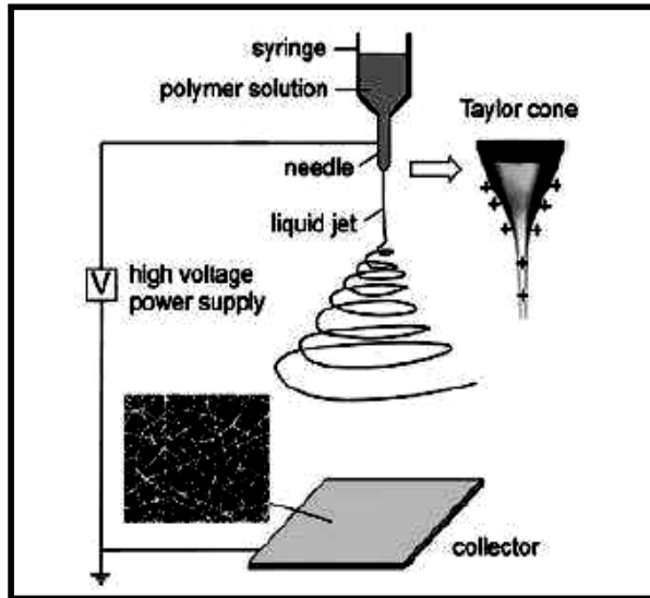
Figure 1. Basic Electrospinning Process
