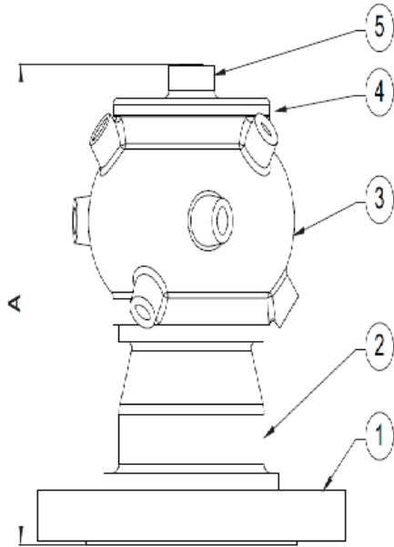
Fig: 2-D Model Of Multi-Nozzle Fire Extinguisher
